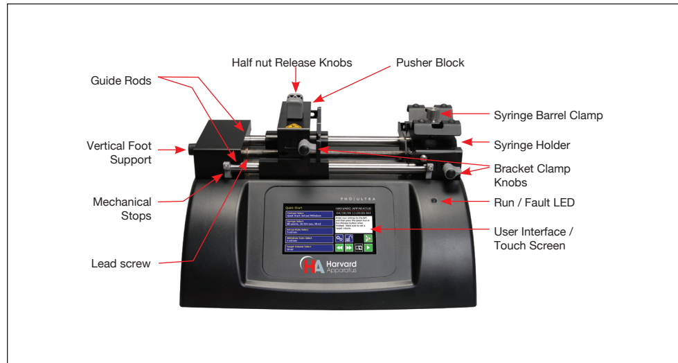
Front view of the PHD ULTRA™ pump showing important components and controls.
