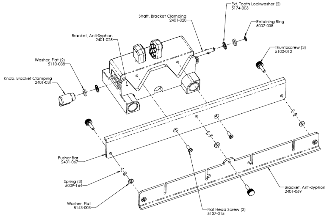
4x140 Multi-Rack Pusher Block Assembly.
