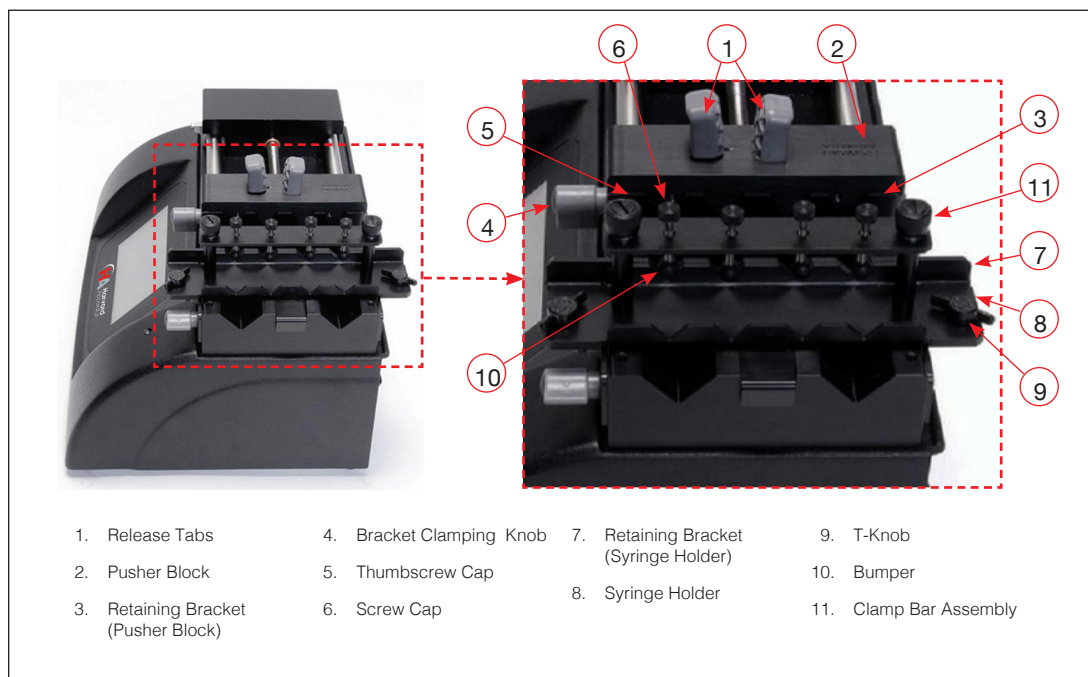
Front view of PHD ULTRA™ showing controls for microliter multi-rack syringe loading.
