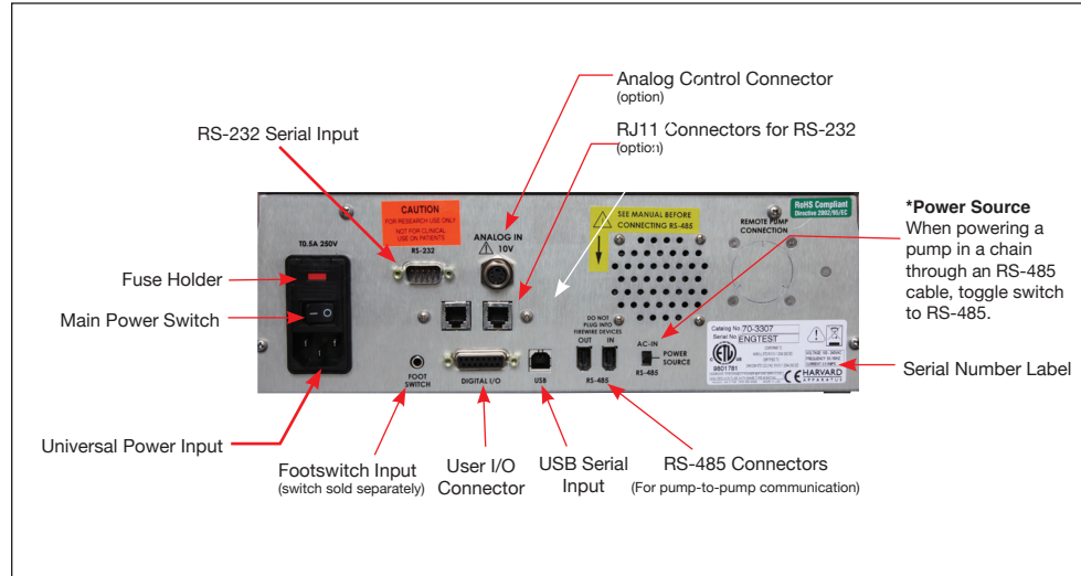
Rear view of the PHD ULTRA™ pump showing important connections.
