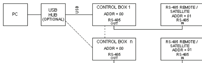
PC Control configuration option
